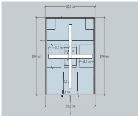
Gambar 3. Desain (2D) rotary slasher
